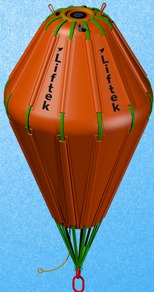
Design of PSAB-2MT to PSAB-50MT
